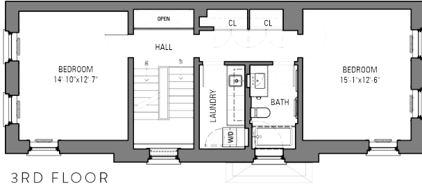
3RD FLOOR
