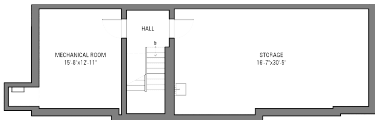
CELLAR FLOOR
